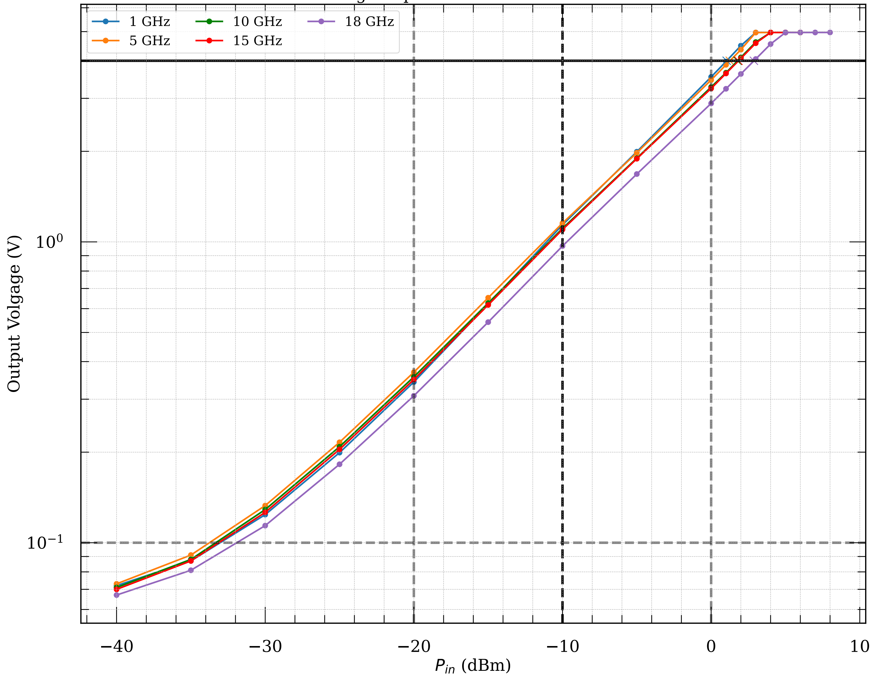
Measured voltage-to-power curve of detector module041v2
